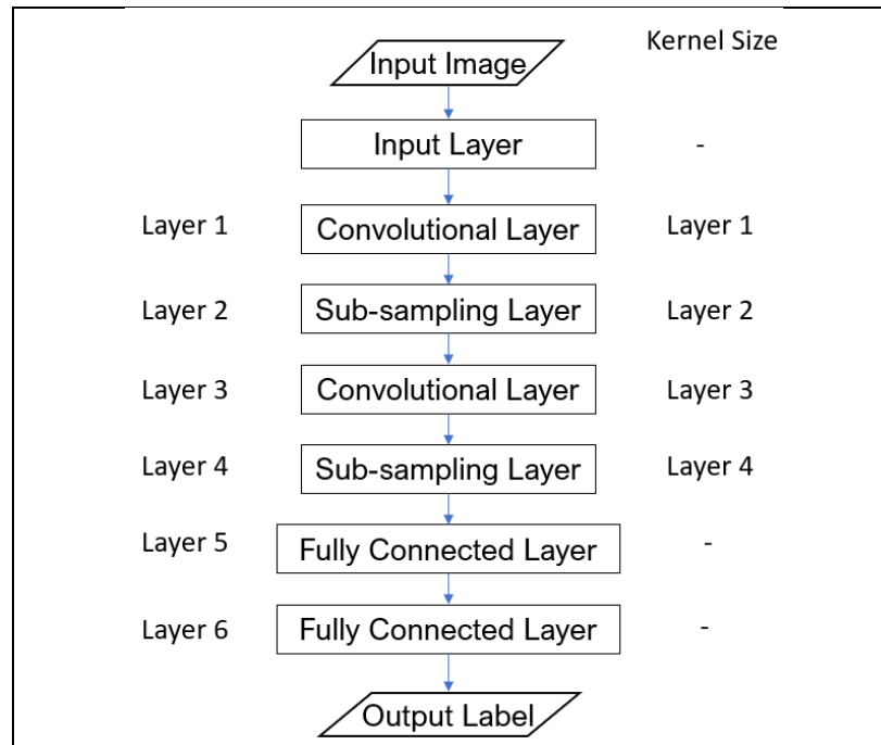
Figure 3: Architecture of the proposed CNN model
