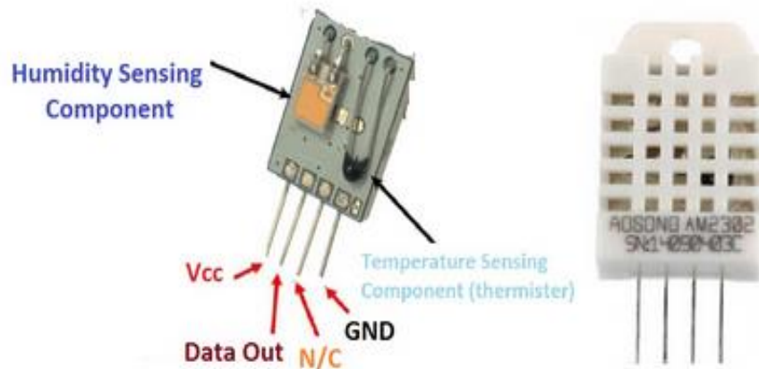
Figure 4: DHT 22 Temperature and Humidity Sensor
