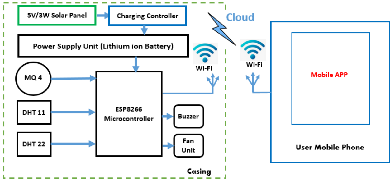
Figure 1: Block Diagram
