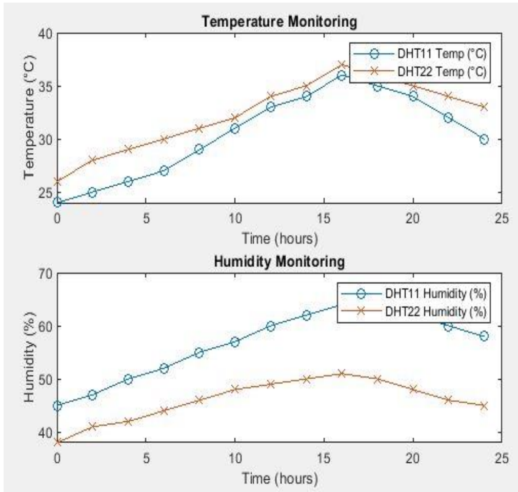
Figure 7: Temperature and Humidity Monitoring for DHT11 and DHT22
