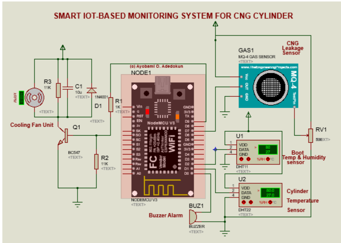
Figure 5: Circuit Simulation Diagram
