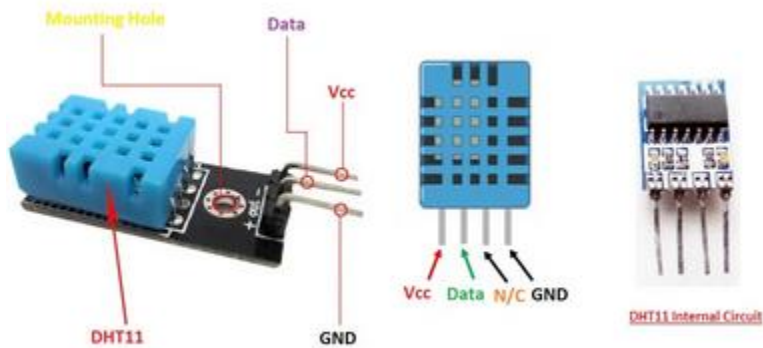
Figure 3: DHT11 Temperature and Humidity Sensor
